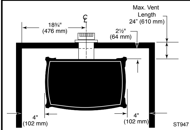
Fig. 3 Parallel Installation, minimum back and side clearance.
