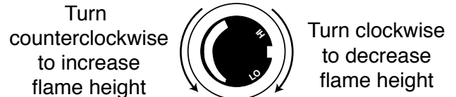
Fig. 65 Flame adjustment knob for SIT valve.
