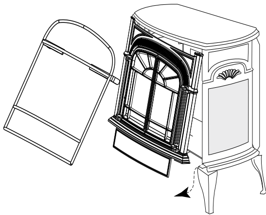
Fig. 82 Remove the safety barrier and stove front.
