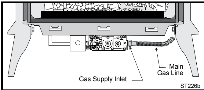
Fig. 68 Attach the gas line to the right side of the valve.
