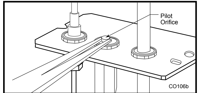
Fig. 78 Remove pilot orifice.
