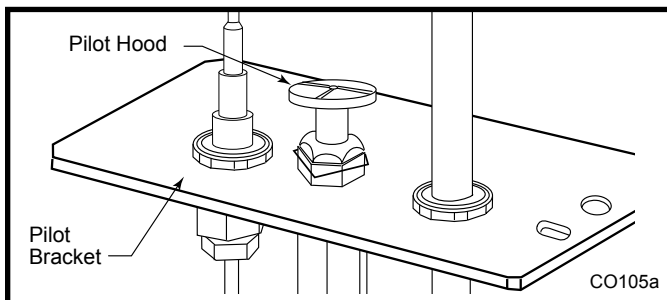
Fig. 75 Remove pilot hood.
