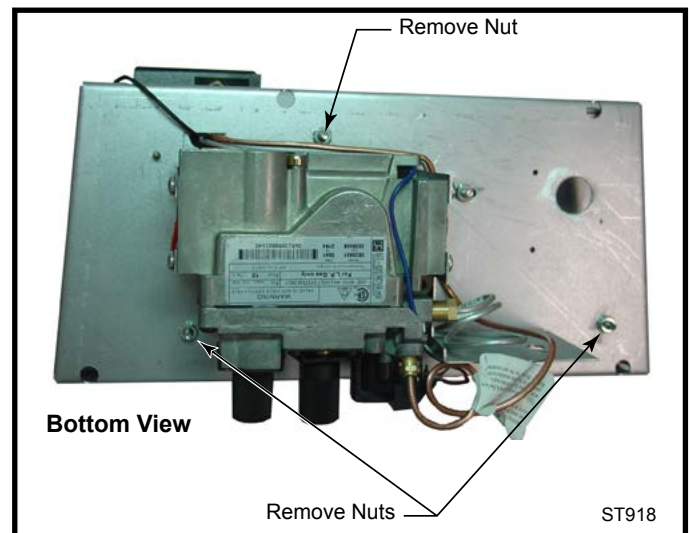
Fig. 79 Remove three (3) nuts securing ember bed in place.
