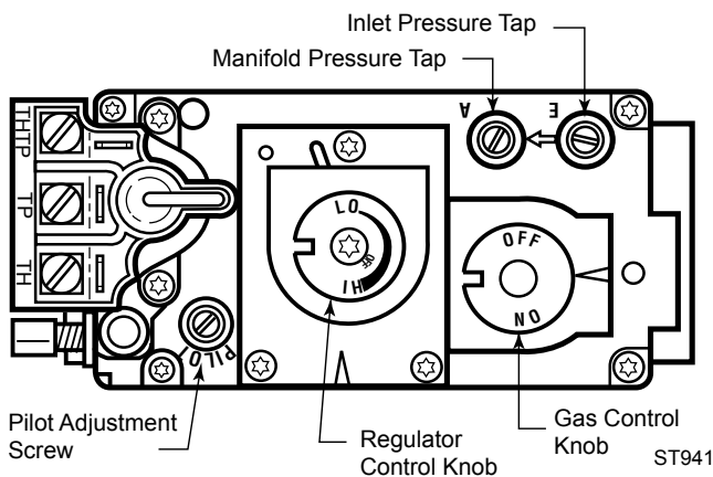
Fig. 63 NOVA SIT valve control.
