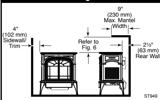
Fig. 5 Alcove and ceiling clearances.
