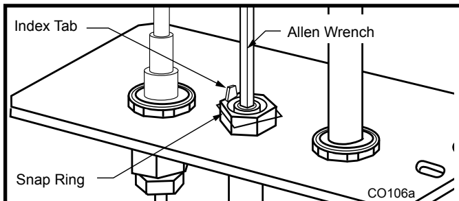
Fig. 76 Remove pilot orifice.
