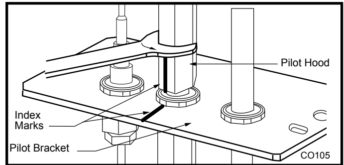
Fig. 77 Remove pilot hood. (Your pilot may have a different appearance.)
