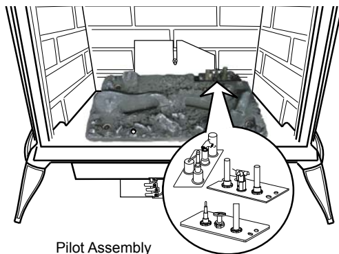
Fig. 64 Pilot Assembly location.
