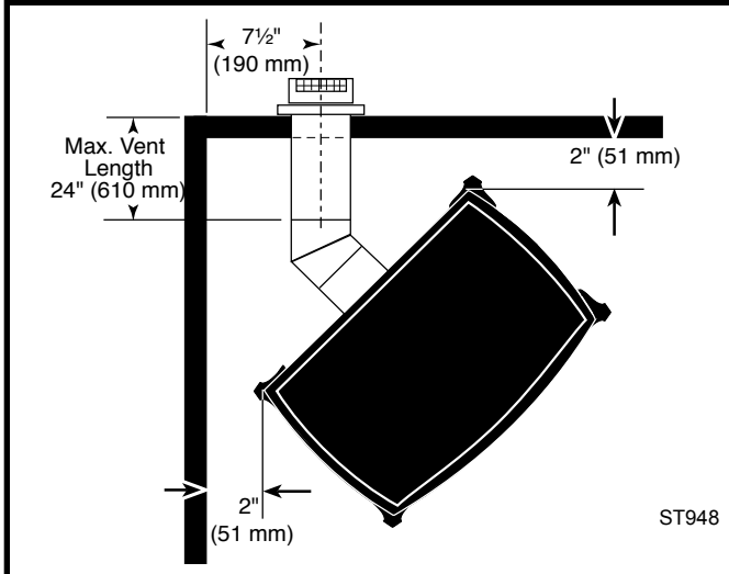
Fig. 4 Corner installation, minimum corner clearance and flue centerline.
