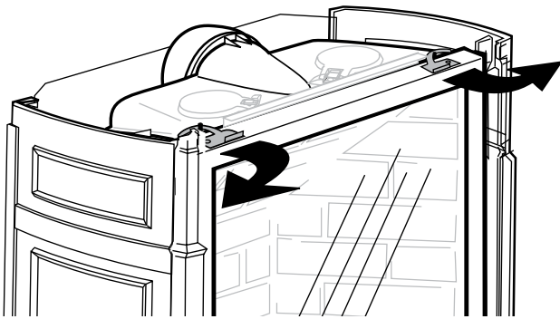
Fig. 83 Release the latches to release the glass frame.
